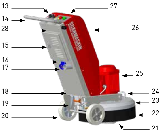
Figure 1.5 Scanmaskin 450NS overview
