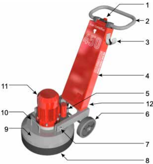
Figure 1.4 Scanmaskin 450 overview
